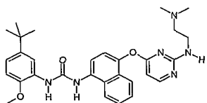
1-(5-tert-Butyl-2-methoxy-phenyl)-3-{4-[2-(2-dimethyl-amino-ethyl-amino)-pyrimidin-4-yloxy]-naphthalen-1-yl}-urea;
